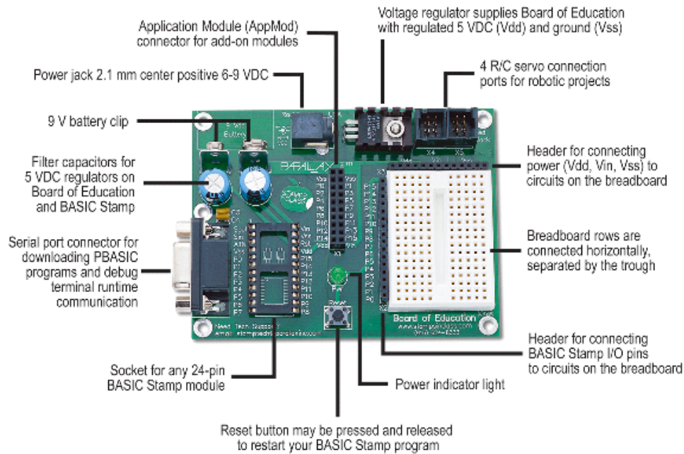
Figure B-4 Board of Education Rev B
