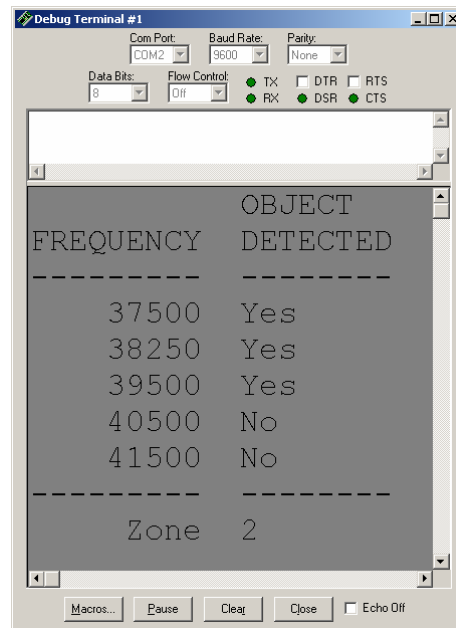
Figure 8-3 Testing Distance Detection
