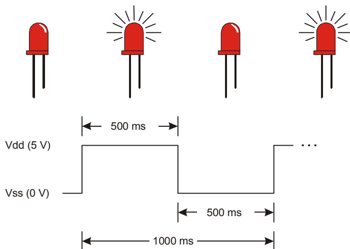
Figure 2-7 Timing Diagram for HighLowLed.bs2
