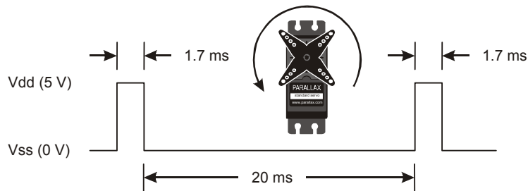
Figure 2-26 A 1.7 ms Pulse Train Makes the Servo Turn Full Speed Counterclockwise
