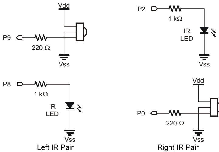
Figure 7-4 Left and Right IR Pairs
