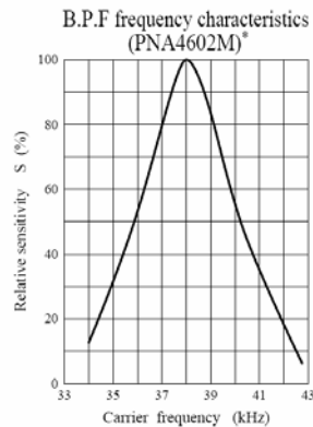
Figure 8-1 Filter Sensitivity
