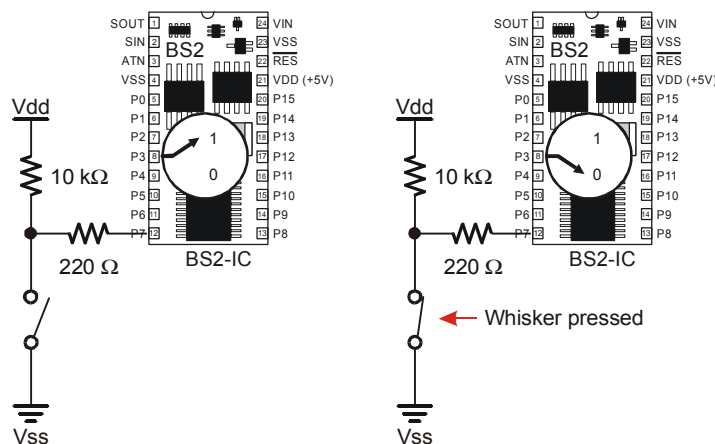
Figure 5-8 Detecting Electrical Contacts
