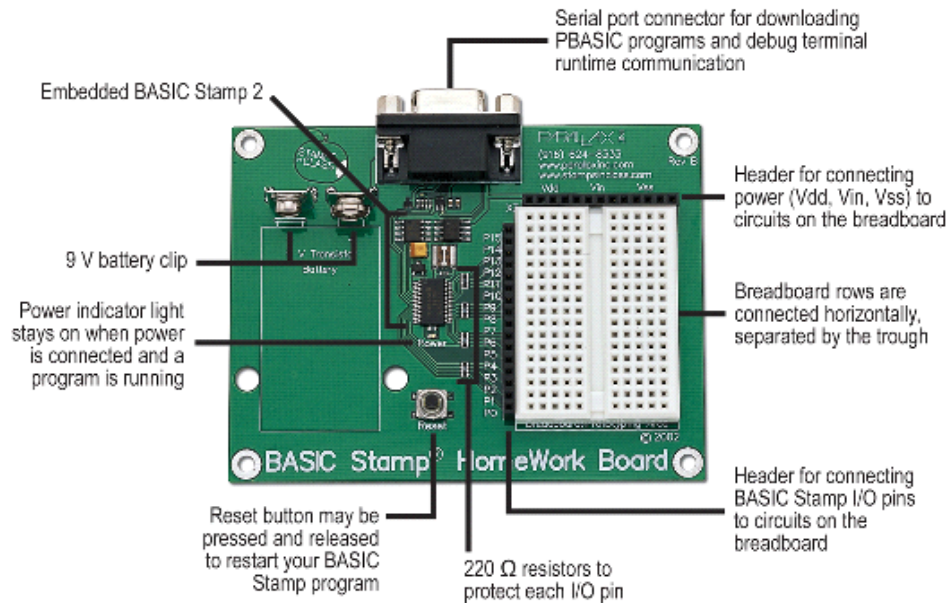
Figure B-3 BASIC Stamp HomeWork Board
