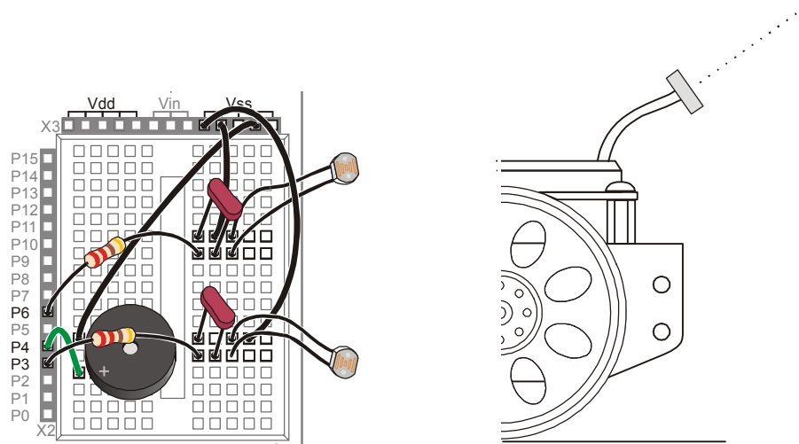
Figure 6-12: Photoresistor Orientation
