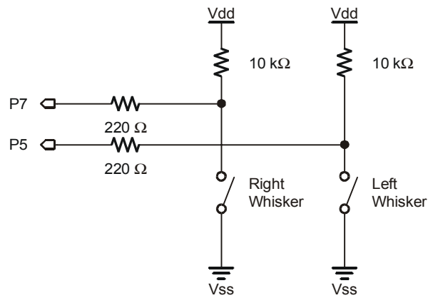
Figure 5-4 Whiskers Schematic.
