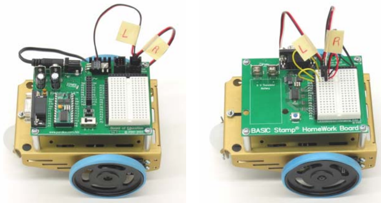
With Board of Education Rev C
