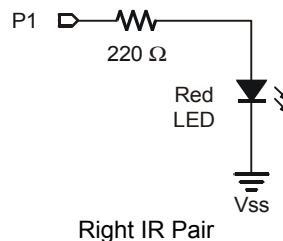
Figure 7-6 Left and Right Indicator LEDs
