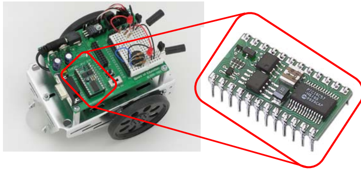
Figure 1-1 BASIC Stamp on a Boe-Bot
