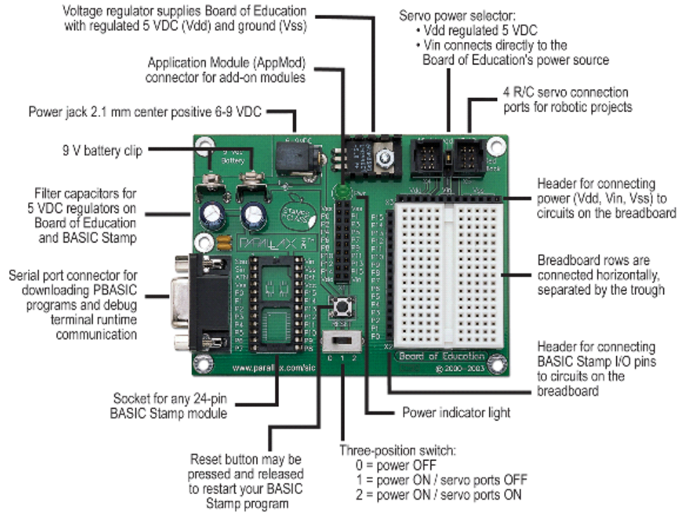
Figure B-2 Board of Education Rev C
