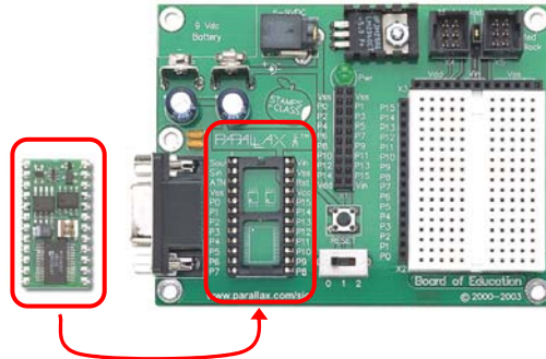
Figure 1-2 BASIC Stamp 2 (left) and Board of Education (right)
