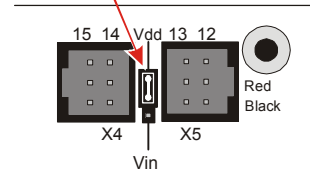
Figure 2-12 Selecting Your Servo's Power Supply on the Board of Education Rev C
