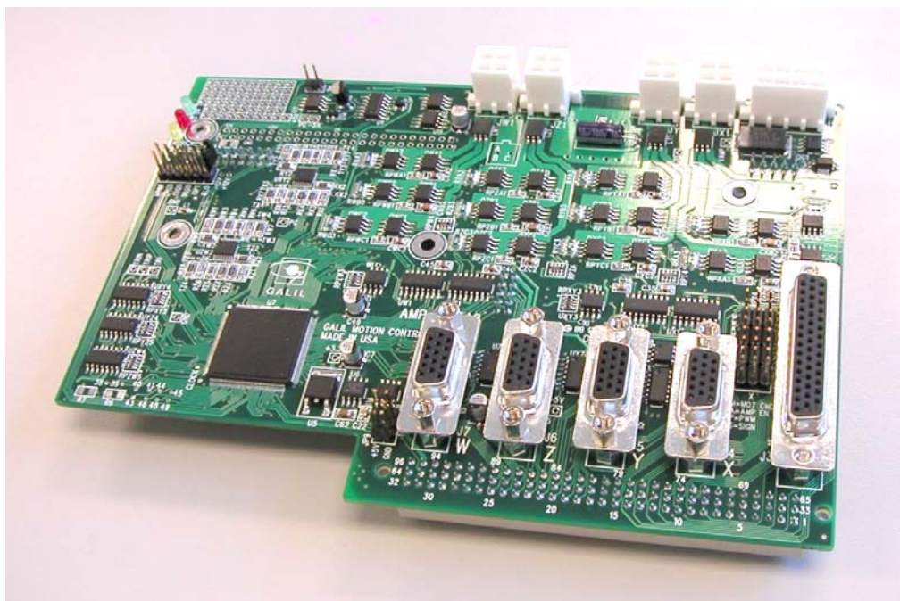
Figure 29 AMP-20542 PWM Servo Amplifier
