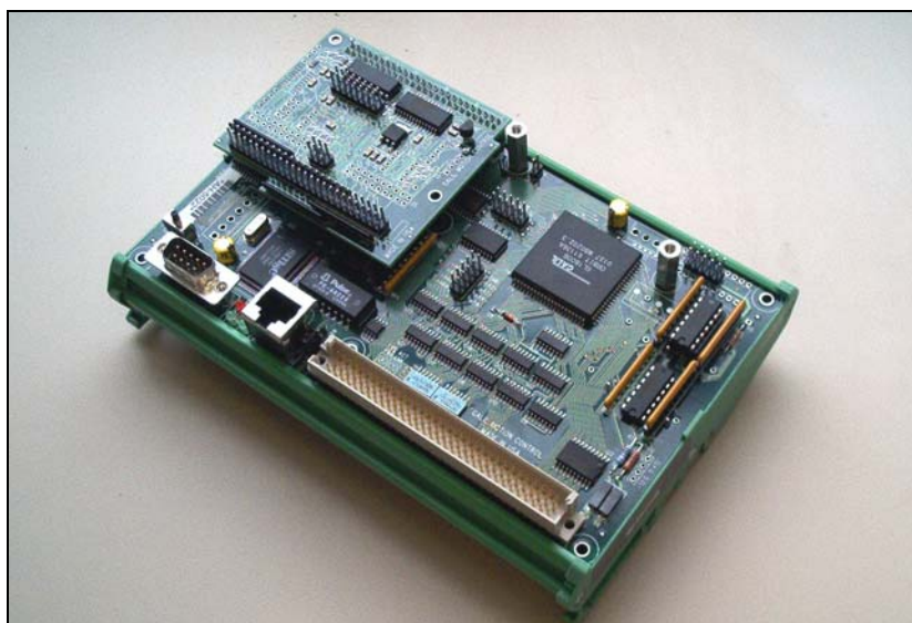
Figure 35 DB-28040 Mounted to DMC-2143-DIN
