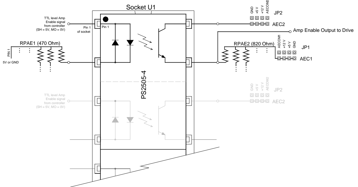
Figure 9 Amplifier Enable Circuit Sourcing Output Configuration
