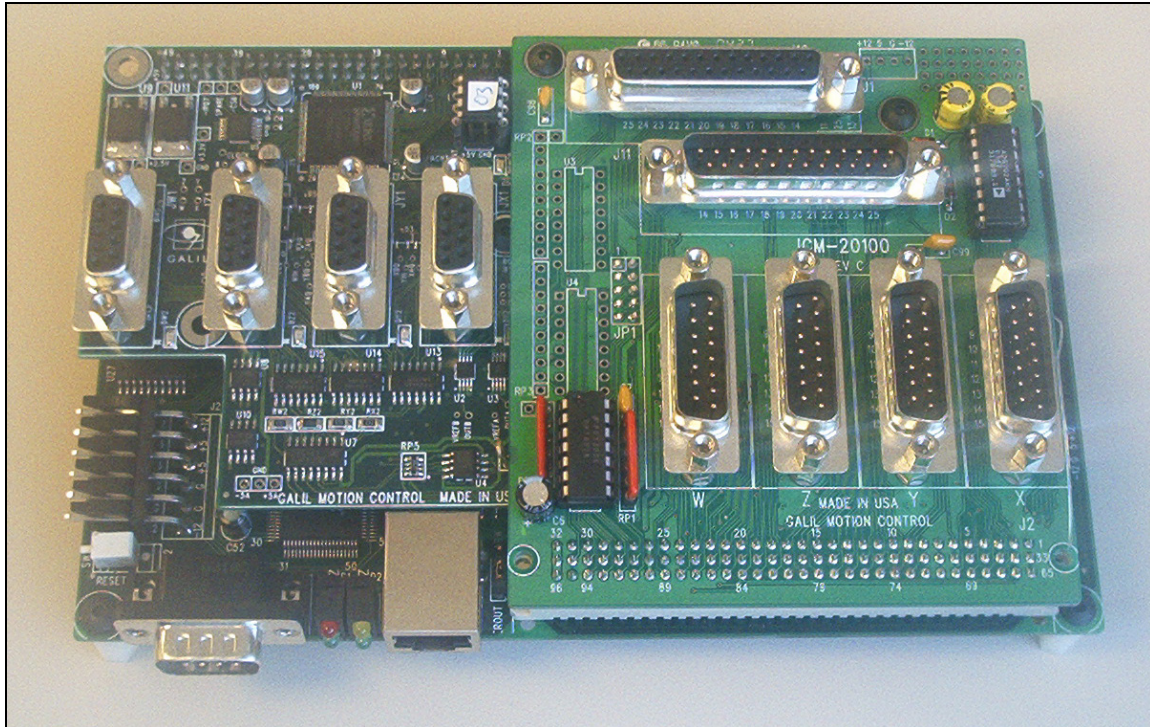
Figure 2- DMC-2143+ICM-20100+DB-28104
