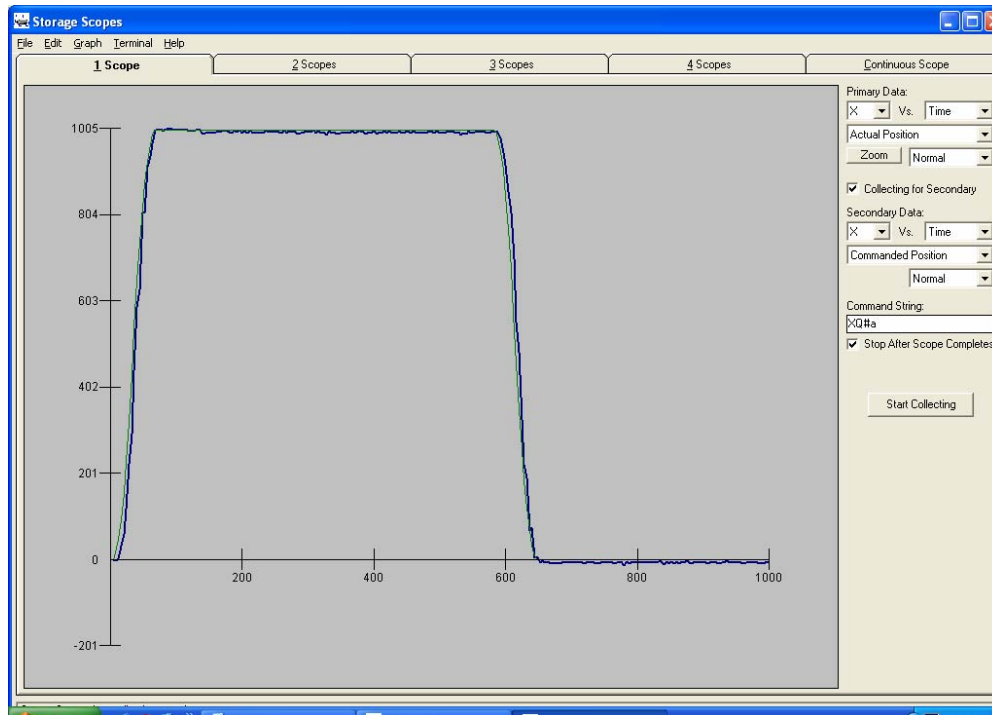
Figure 7- AFX=12 step response.
