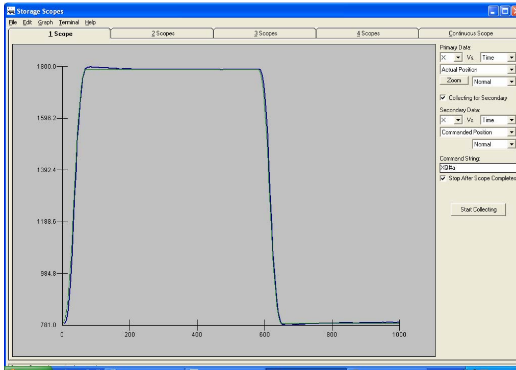
Figure 6- AFX=10 Step Response
