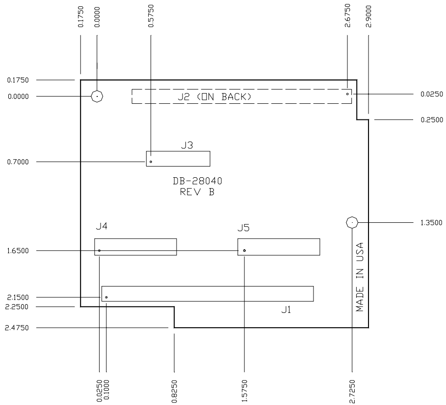
Figure 36 DB-28040 Interconnect Mounting Dimensions Overall Dimensions: 3.075" x 2.650"
