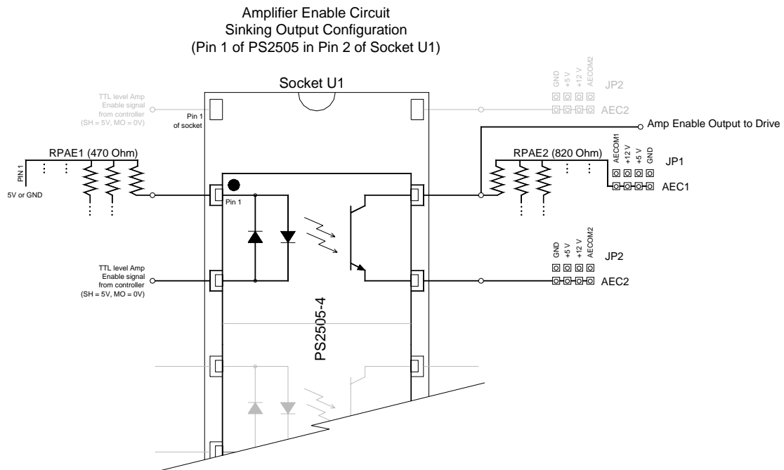
Figure 8 Amplifier Enable Circuit Output Configuration
