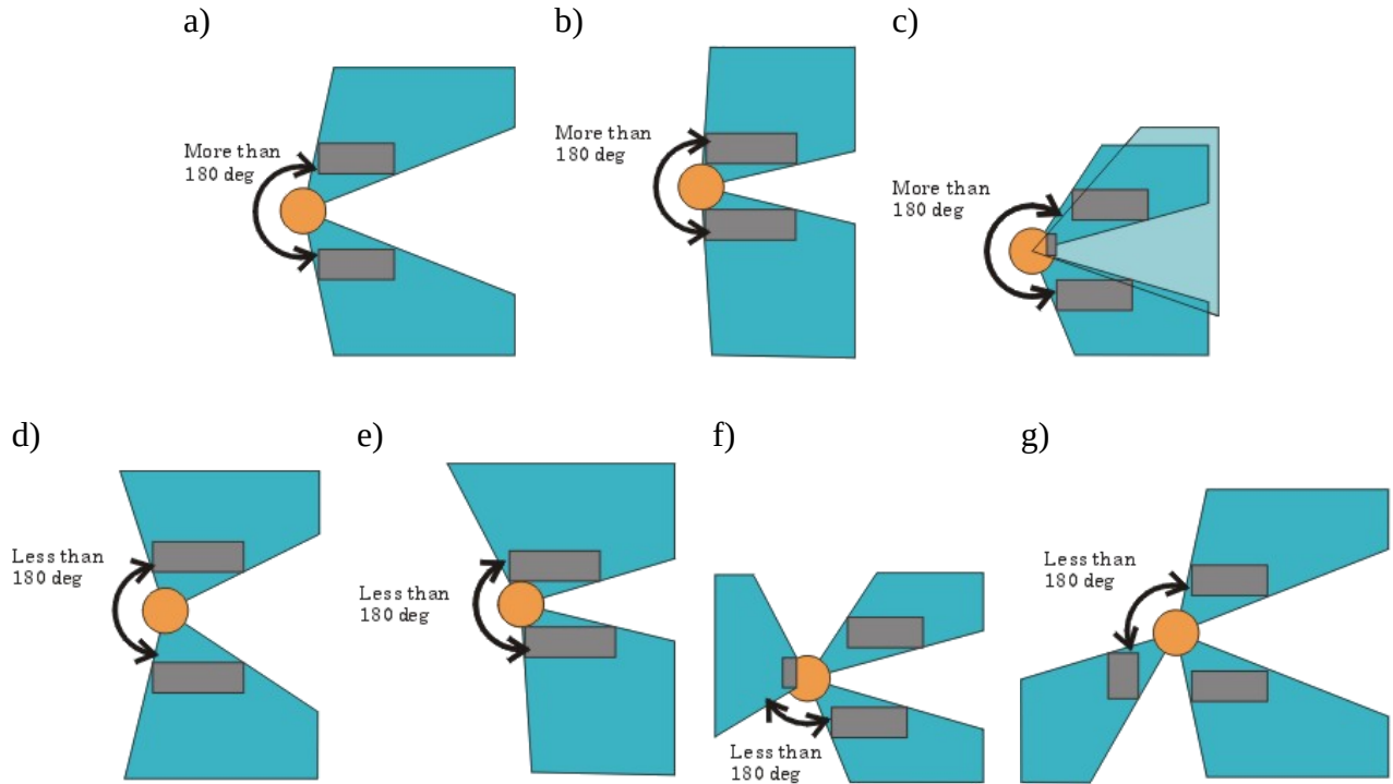
Figure 9: Examples for “Ball Holding”. The orange circle is the ball, the gray boxes are parts of the robot, and the blue area visualizes the ranges occupied by the robot. Situations a), b) and c) are legal, whereas d), e), f) and g) violate the rule.
